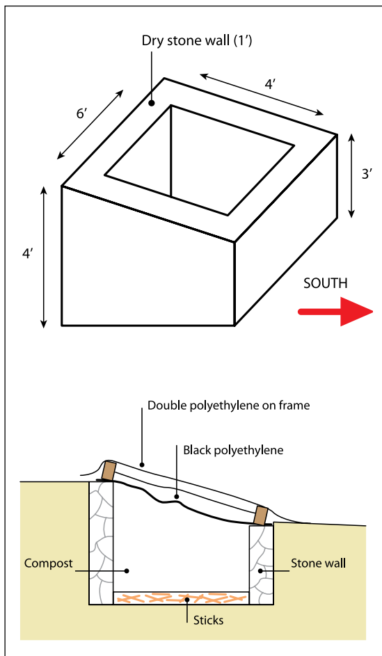
Figure 21: Compost trench designed for cold climates. Walls are not cemented to allow good air circulation.
