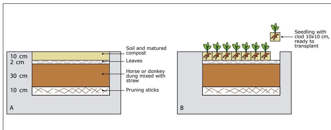
Figure 10: nursery production. Hot bed
