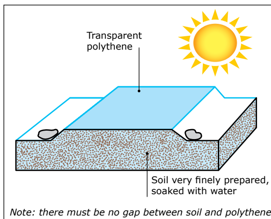
Figure 18: disinfecting soil by solar heating
