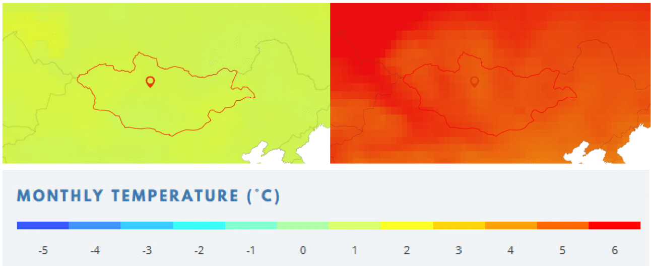
Figure 26: Temperature projections for Arkhangai - 2080-2099 - RCP2.6 vs. RCP8.5
