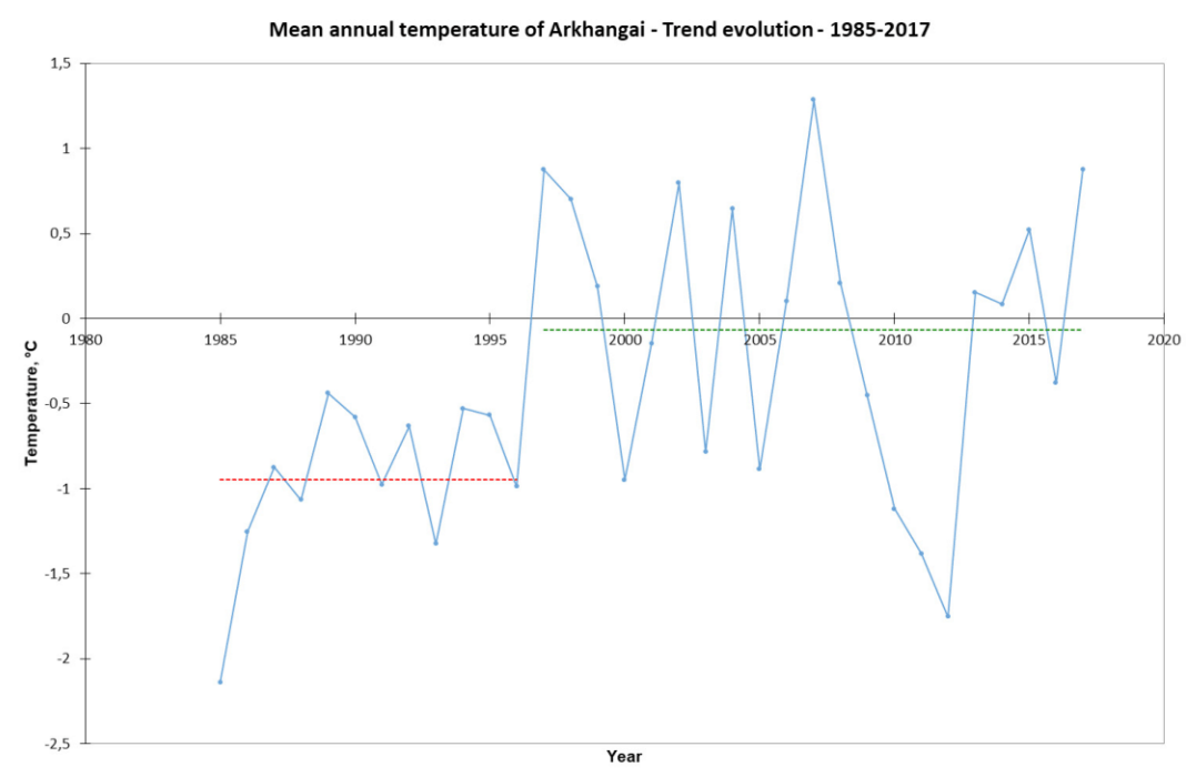
Figure 18: Trend analysis of mean annual temperature evolution
