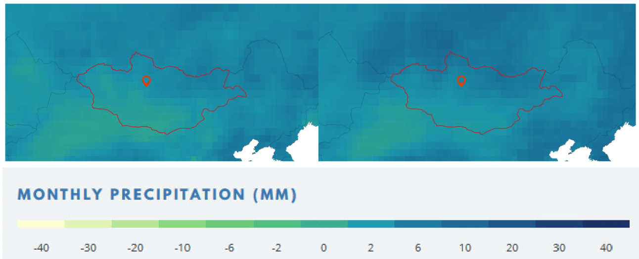
Figure 27: Precipitation projections for Arkhangai - 2040-2059 - RCP2.6 vs. RCP8.5
