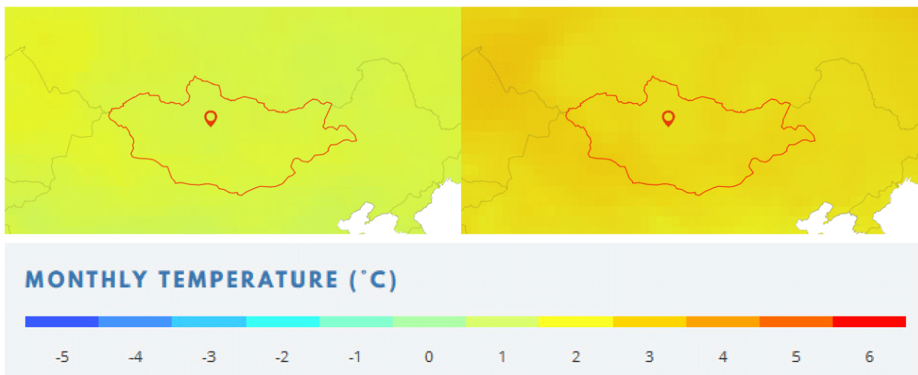
Figure 25: Temperature projections for Arkhangai - 2040-2059 - RCP2.6 vs. RCP8.5
